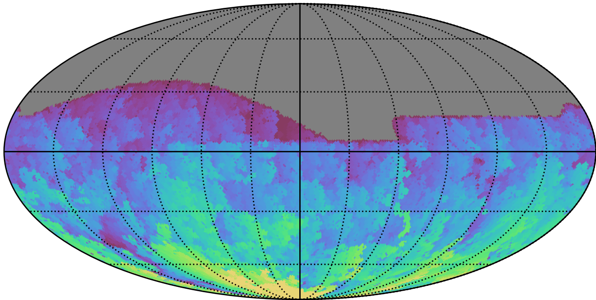
ddf_acor_sf20_lsf30_lsr20_v3.4_10yrs All sky g band: Max HA
