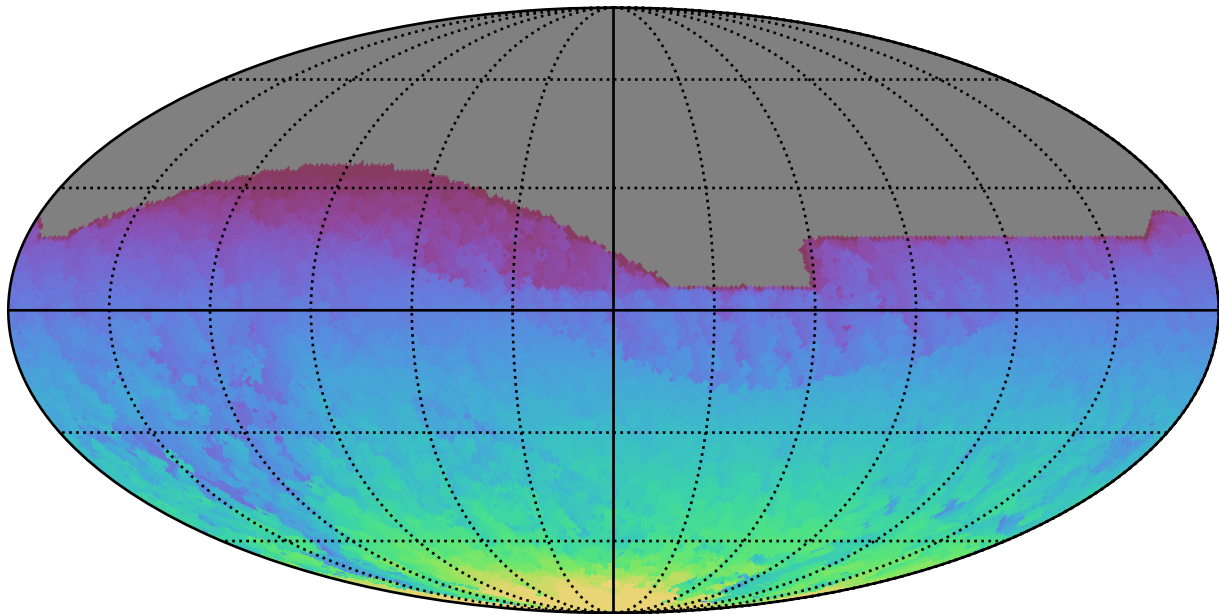
ddf_acor_sf20_lsf30_lsr20_v3.4_10yrs All sky all bands: Max HA
