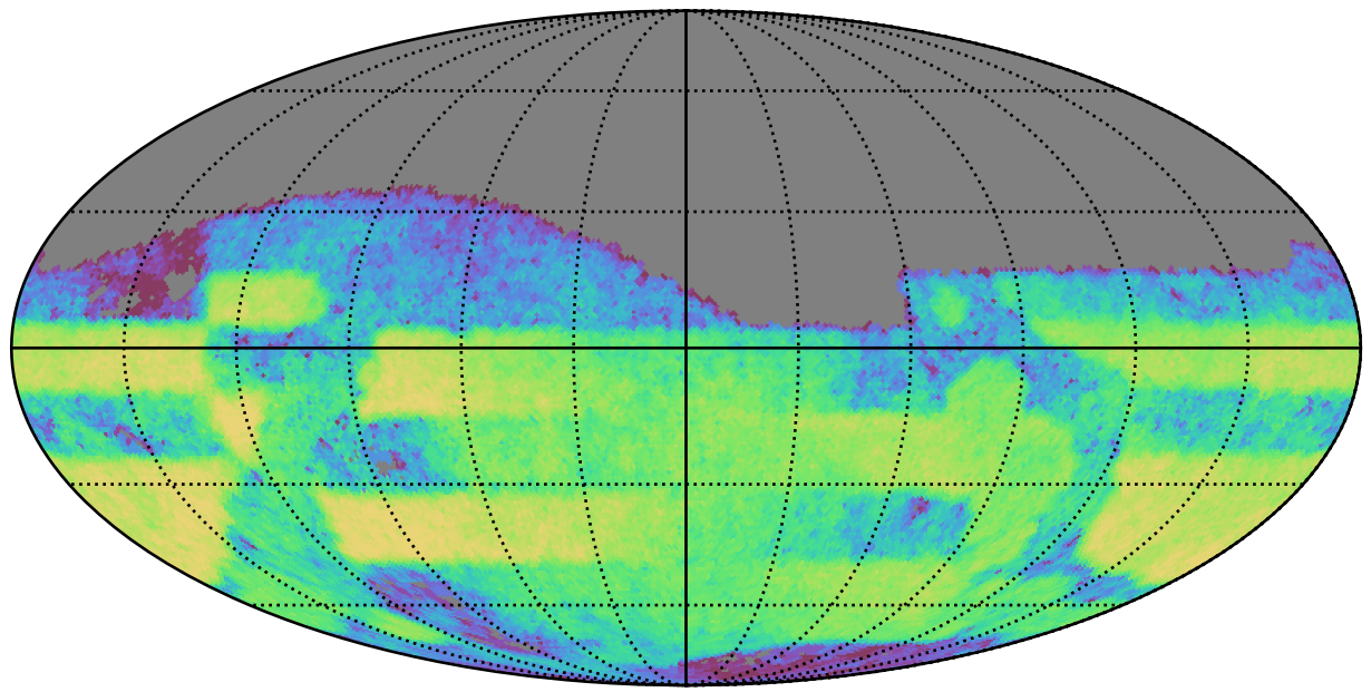
ddf_acor_sf20_lsf30_lsr20_v3.4_10yrs Yr 3-4 i band: CoaddM5
