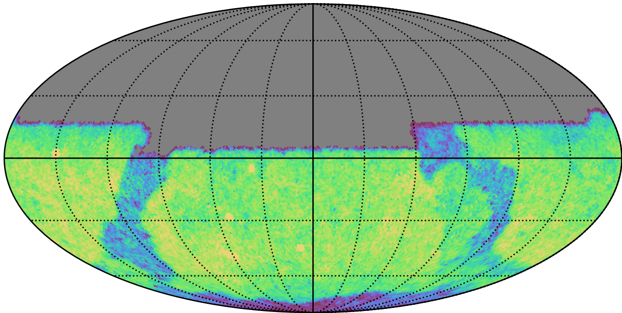
ddf_acor_sf20_lsf30_lsr20_v3.4_10yrs Yr 1 y band: CoaddM5
