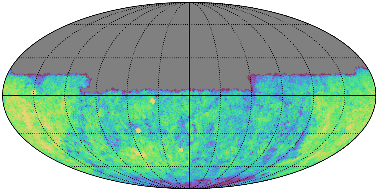
ddf_acor_sf20_lsf30_lsr20_v3.4_10yrs Yr 1 u band: CoaddM5
