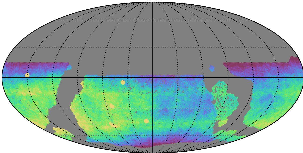
ddf_acor_sf20_lsf30_lsr20_v3.4_10yrs WFD r band: CoaddM5
