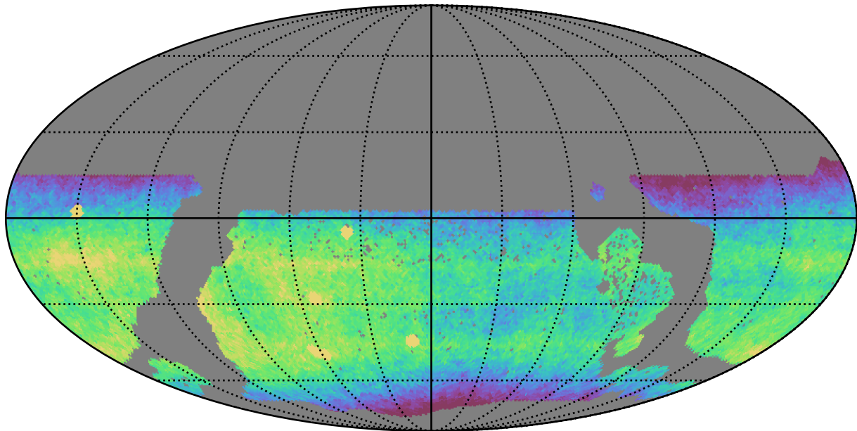
ddf_acor_sf20_lsf30_lsr20_v3.4_10yrs WFD i band: CoaddM5
