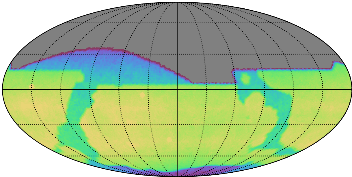
ddf_acor_sf20_lsf30_lsr20_v3.4_10yrs All sky i band: CoaddM5
