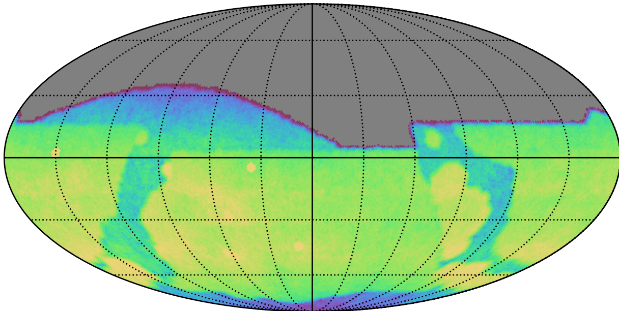
ddf_acor_sf20_lsf30_lsr20_v3.4_10yrs All sky g band: CoaddM5
