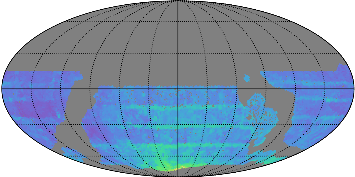
ddf_acor_sf20_lsf30_lsr20_v3.4_10yrs WFD all bands: 80thPercentile Season Length
