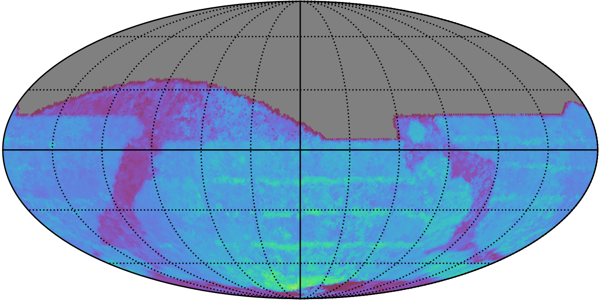
ddf_acor_sf20_lsf30_lsr20_v3.4_10yrs All sky z band: 80thPercentile Season Length
