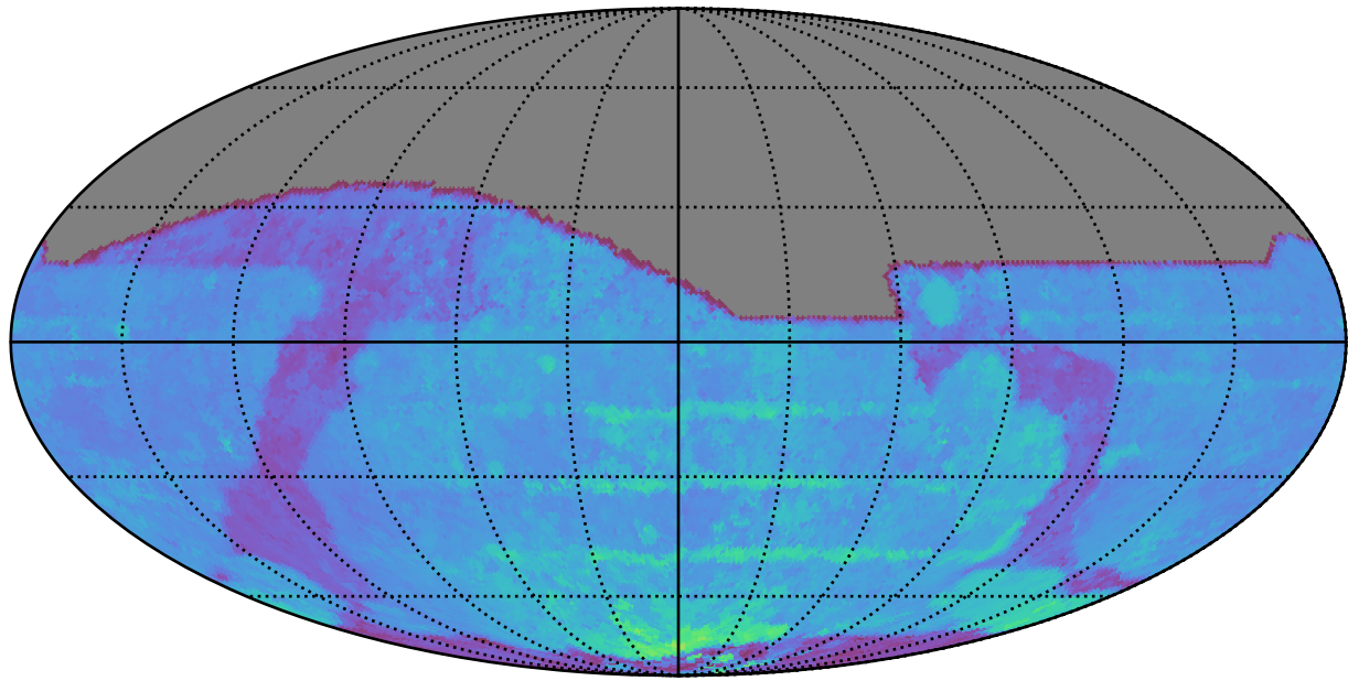
ddf_acor_sf20_lsf30_lsr20_v3.4_10yrs All sky i band: 80thPercentile Season Length
