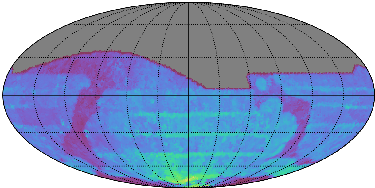
ddf_acor_sf20_lsf30_lsr20_v3.4_10yrs All sky all bands: 80thPercentile Season Length
