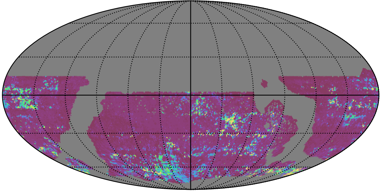
ddf_acor_sf20_lsf30_lsr20_v3.4_10yrs WFD z band: 75th Percentile Intranight Timespan
