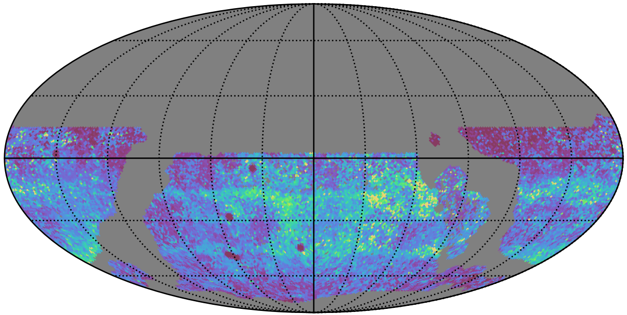
ddf_acor_sf20_lsf30_lsr20_v3.4_10yrs WFD y band: 75th Percentile Intranight Timespan
