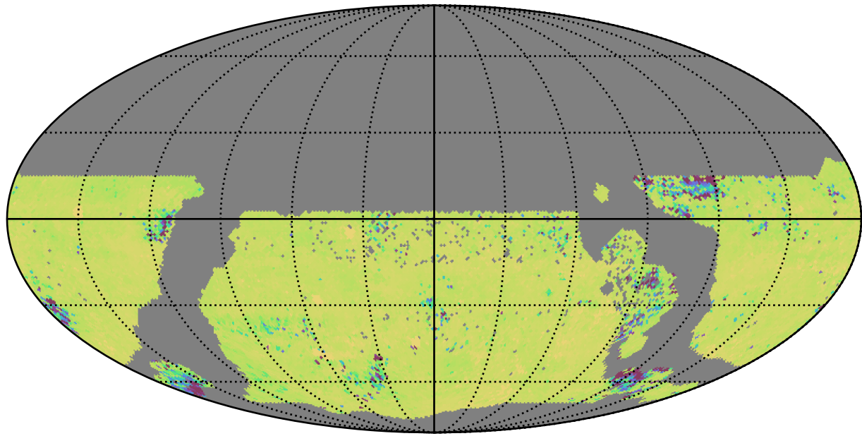
ddf_acor_sf20_lsf30_lsr20_v3.4_10yrs WFD ug bands: 75th Percentile Intranight Timespan
