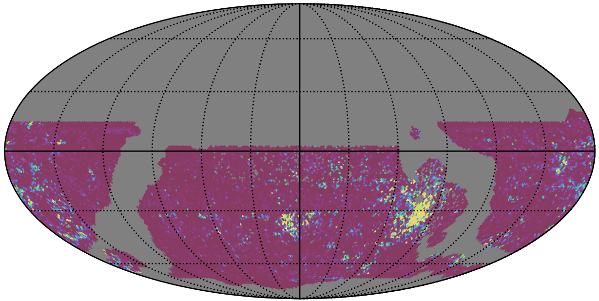
ddf_acor_sf20_lsf30_lsr20_v3.4_10yrs WFD u band: 75th Percentile Intranight Timespan
