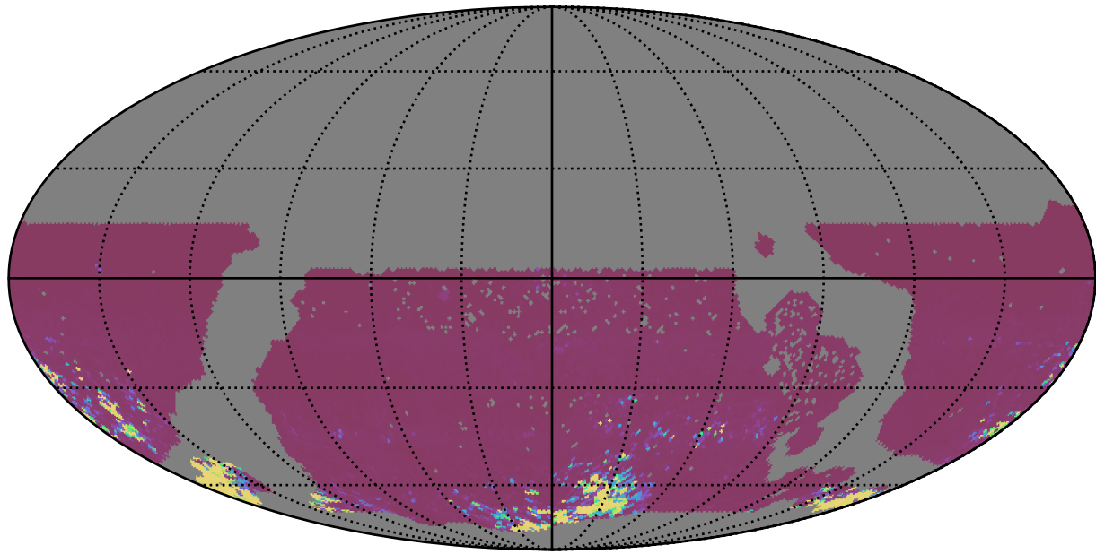
ddf_acor_sf20_lsf30_lsr20_v3.4_10yrs WFD ri bands: 75th Percentile Intranight Timespan
