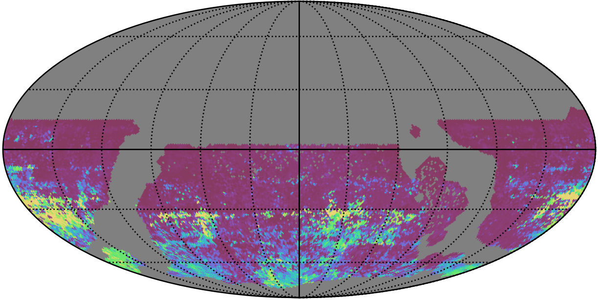
ddf_acor_sf20_lsf30_lsr20_v3.4_10yrs WFD r band: 75th Percentile Intranight Timespan
