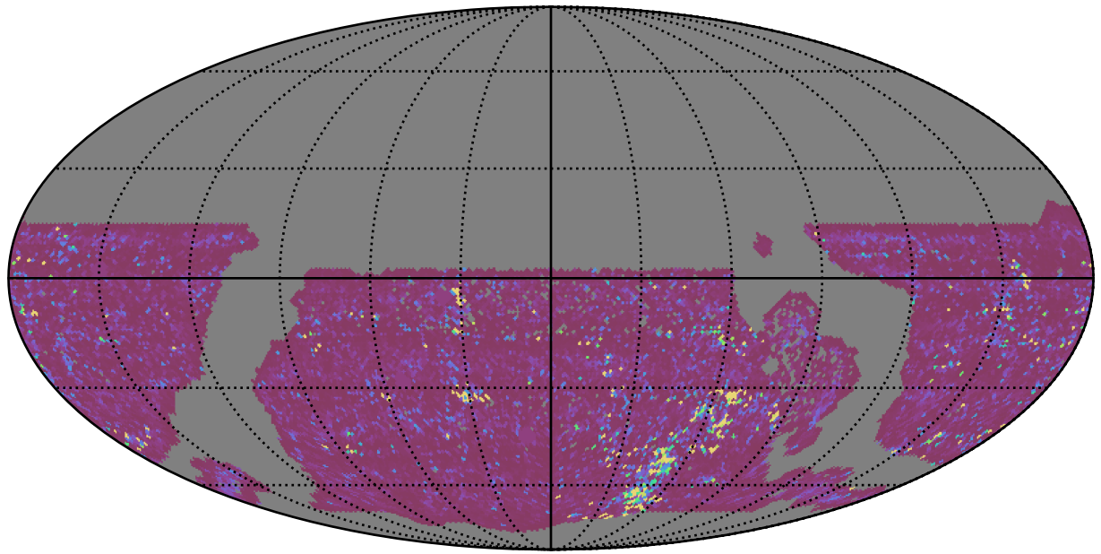
ddf_acor_sf20_lsf30_lsr20_v3.4_10yrs WFD g band: 75th Percentile Intranight Timespan
