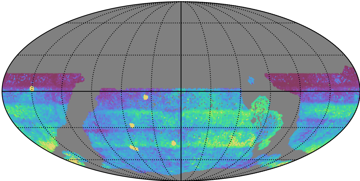
ddf_acor_sf20_lsf30_lsr20_v3.4_10yrs WFD: 75th Percentile Intranight Timespan
