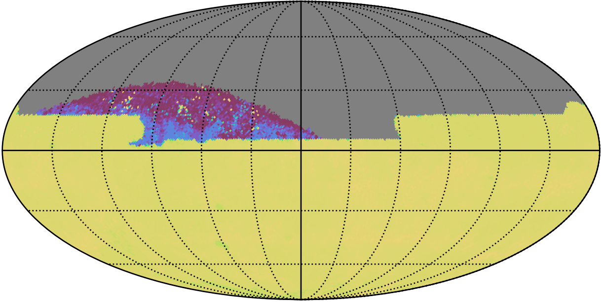
ddf_acor_sf20_lsf30_lsr20_v3.4_10yrs All sky zy bands: 75th Percentile Intranight Timespan
