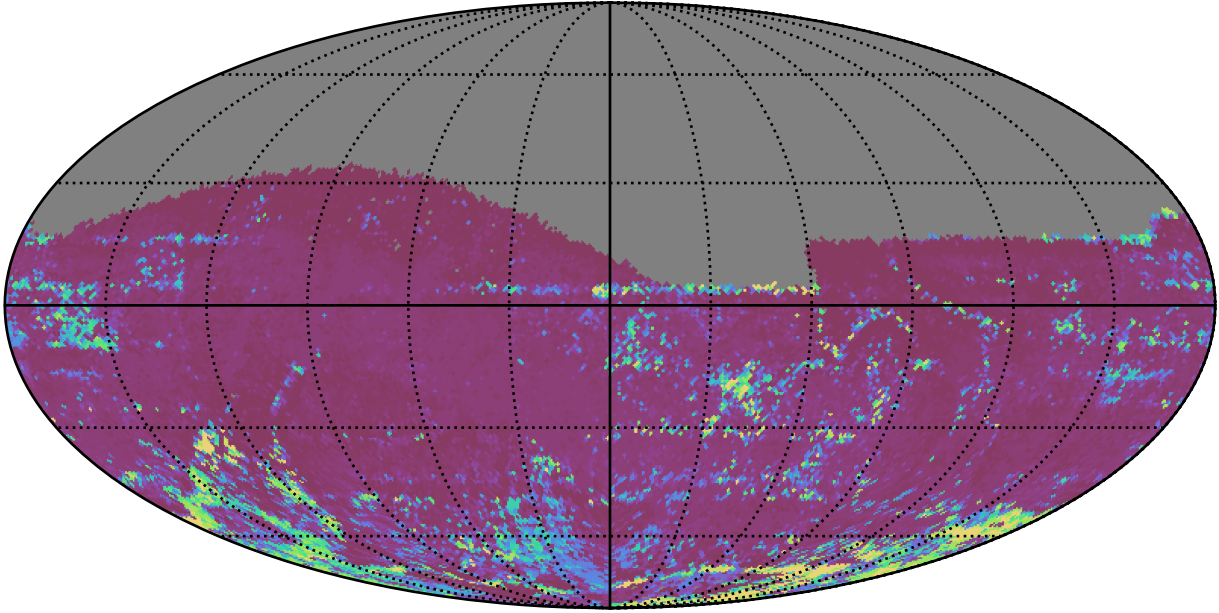
ddf_acor_sf20_lsf30_lsr20_v3.4_10yrs All sky z band: 75th Percentile Intranight Timespan
