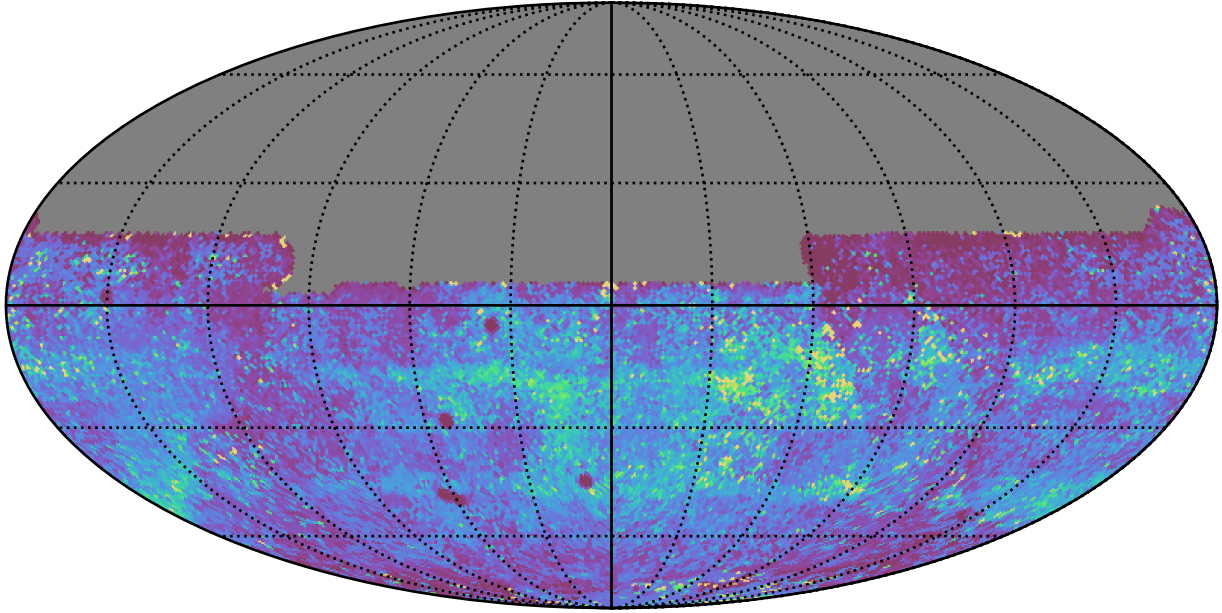
ddf_acor_sf20_lsf30_lsr20_v3.4_10yrs All sky y band: 75th Percentile Intranight Timespan
