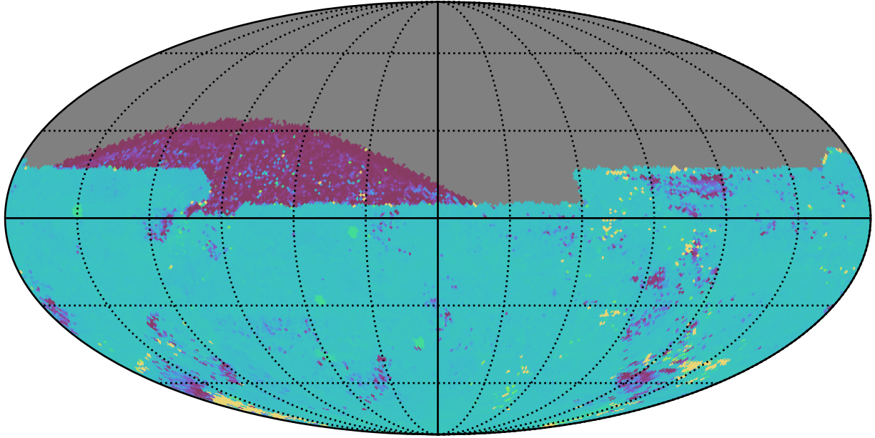
ddf_acor_sf20_lsf30_lsr20_v3.4_10yrs All sky ug bands: 75th Percentile Intranight Timespan
