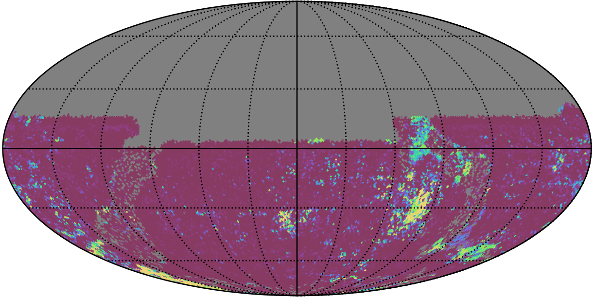
ddf_acor_sf20_lsf30_lsr20_v3.4_10yrs All sky u band: 75th Percentile Intranight Timespan
