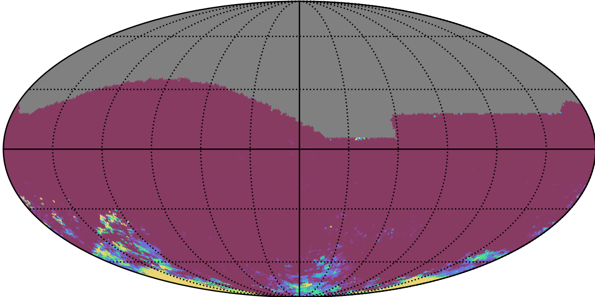
ddf_acor_sf20_lsf30_lsr20_v3.4_10yrs All sky ri bands: 75th Percentile Intranight Timespan
