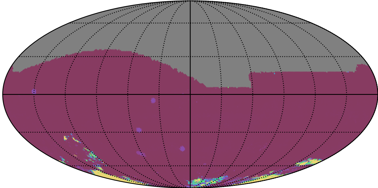
ddf_acor_sf20_lsf30_lsr20_v3.4_10yrs All sky iz bands: 75th Percentile Intranight Timespan
