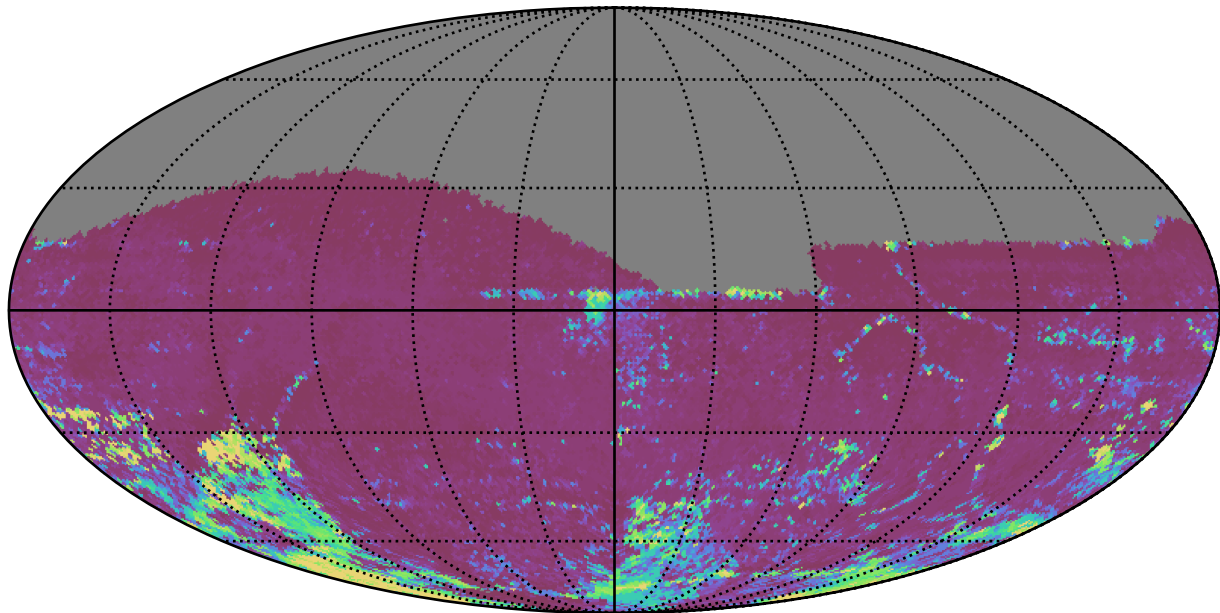
ddf_acor_sf20_lsf30_lsr20_v3.4_10yrs All sky i band: 75th Percentile Intranight Timespan
