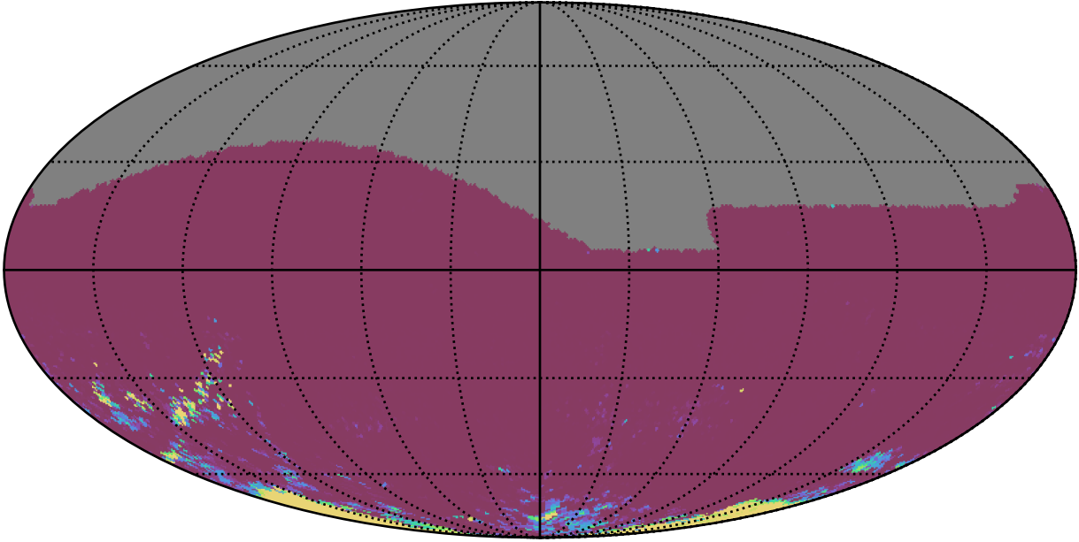
ddf_acor_sf20_lsf30_lsr20_v3.4_10yrs All sky gr bands: 75th Percentile Intranight Timespan
