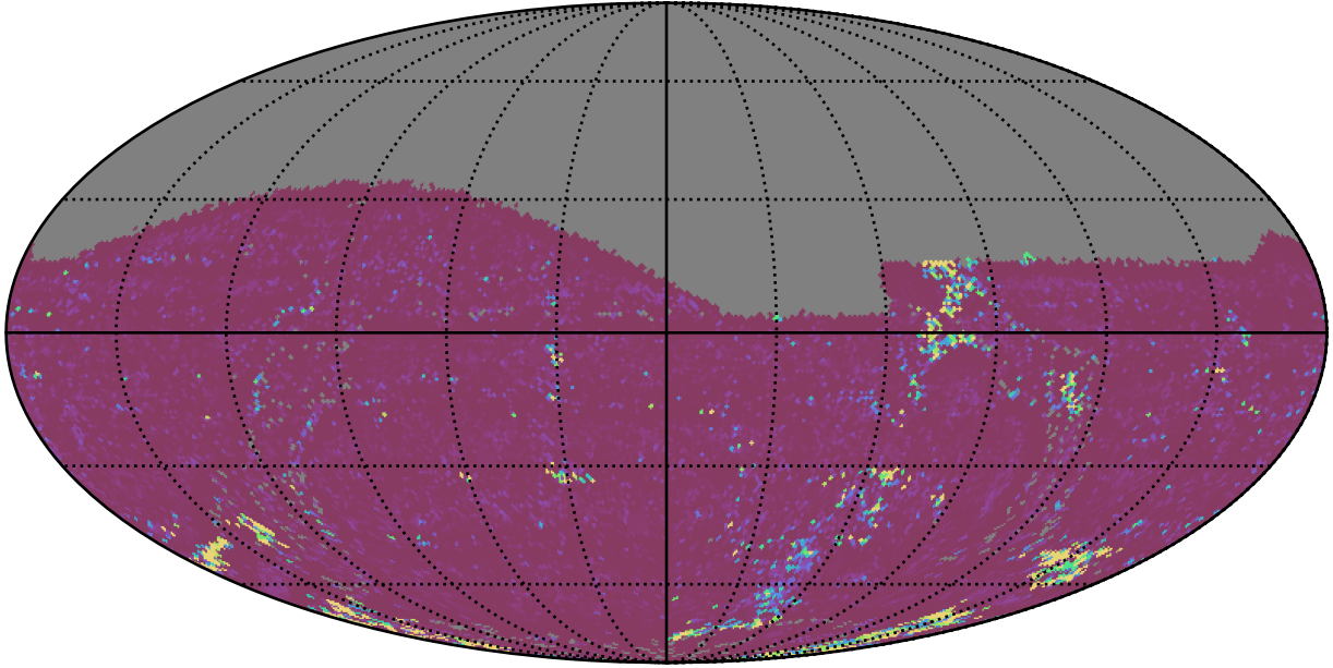
ddf_acor_sf20_lsf30_lsr20_v3.4_10yrs All sky g band: 75th Percentile Intranight Timespan
