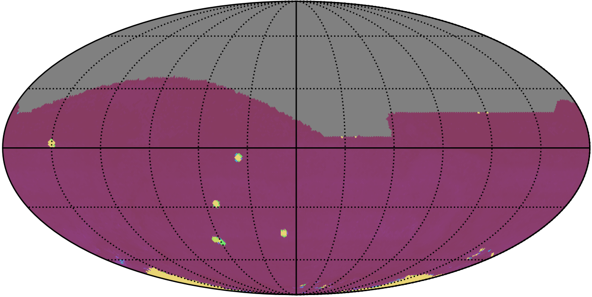
ddf_acor_sf20_lsf30_lsr20_v3.4_10yrs All sky all bands: 75th Percentile Intranight Timespan
