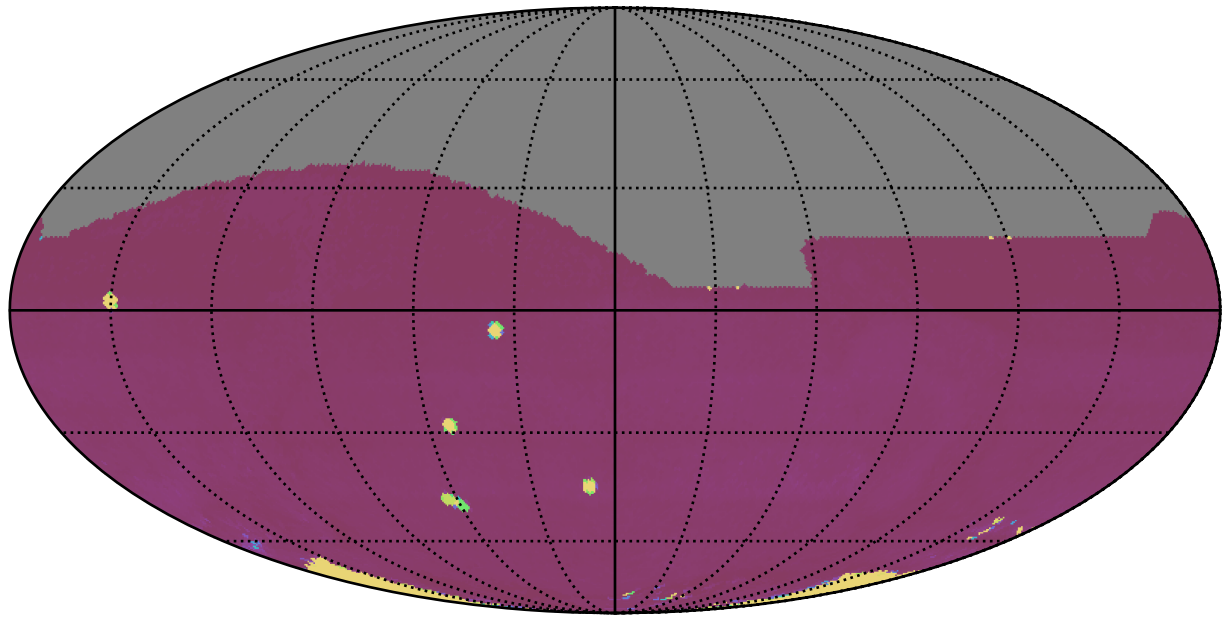
ddf_acor_sf20_lsf30_lsr20_v3.4_10yrs All sky: 75th Percentile Intranight Timespan
