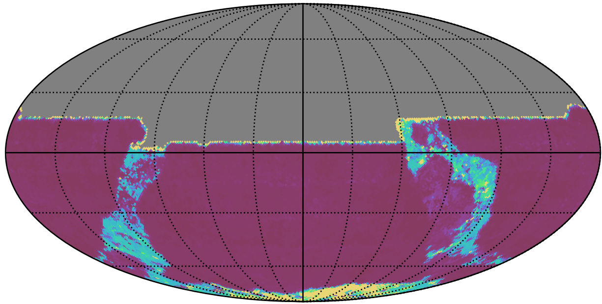
ddf_acor_sf20_lsf30_lsr20_v3.4_10yrs All sky y band: 20thPercentile Inter-Night Gap
