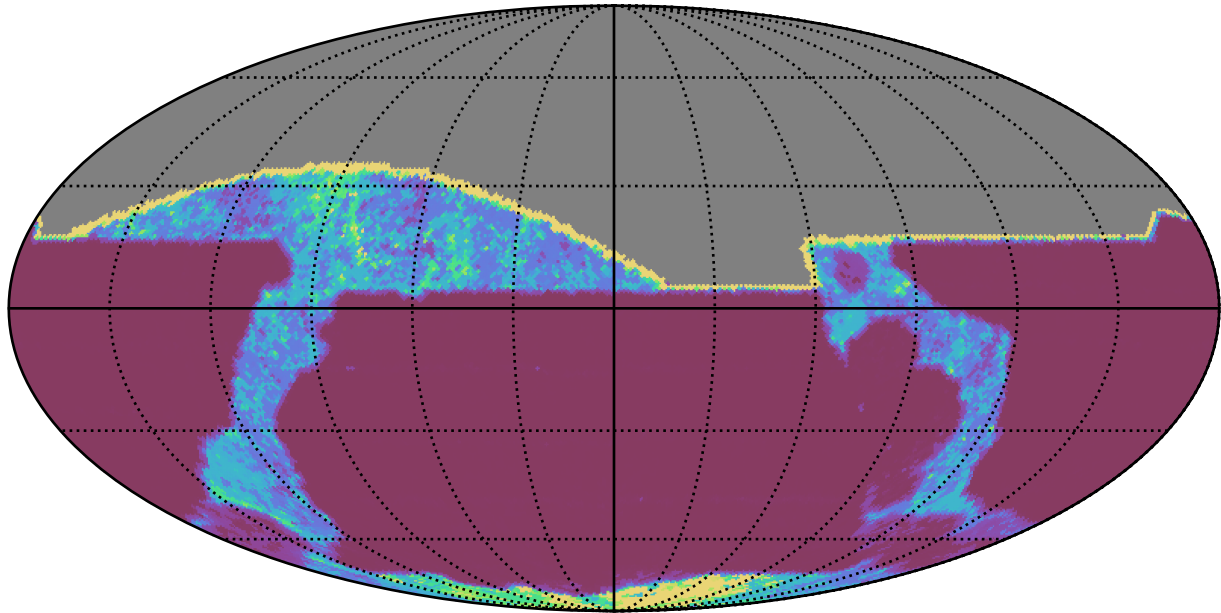
ddf_acor_sf20_lsf30_lsr20_v3.4_10yrs All sky all bands: 20thPercentile Inter-Night Gap
