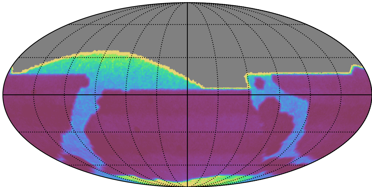
ddf_acor_sf20_lsf30_lsr20_v3.4_10yrs : properMotion
