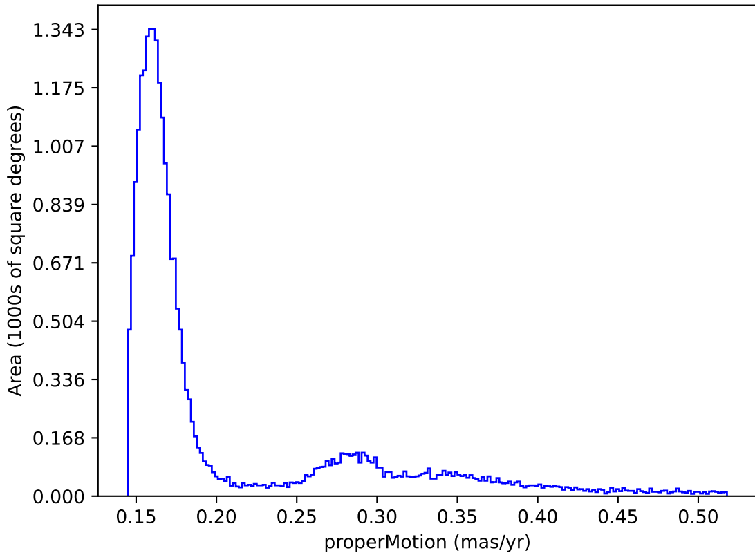
ddf_acor_sf20_ls30_lsr20_v3.4_10yrs : properMotion
