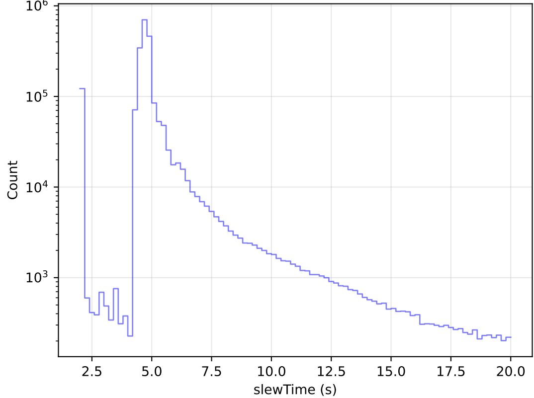
ddf_acor_sf20_Isf30_Isr20_v3.4_10yrs All visits: Zoom Slew Time Histogram
