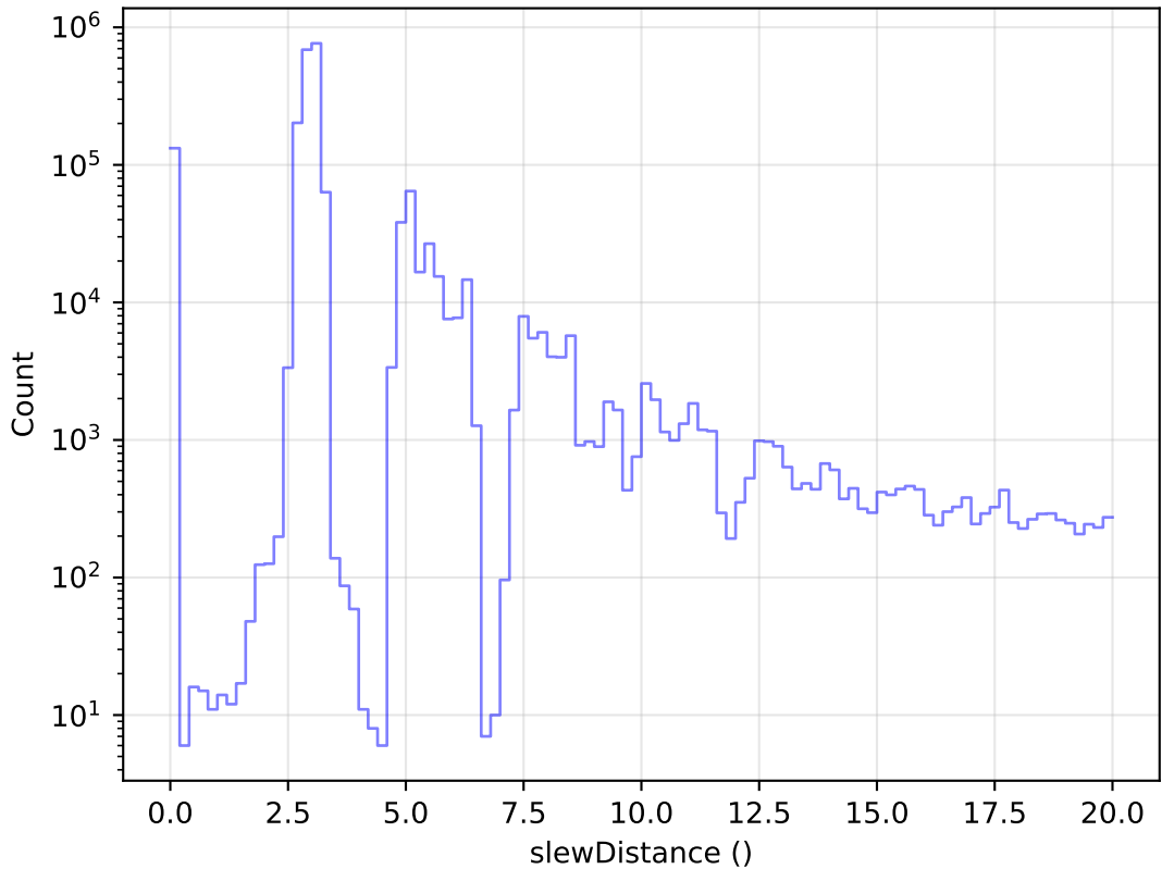
ddf_acor_sf20_lsf30_lsr20_v3.4_10yrs All visits: Zoom Slew Distance Histogram
