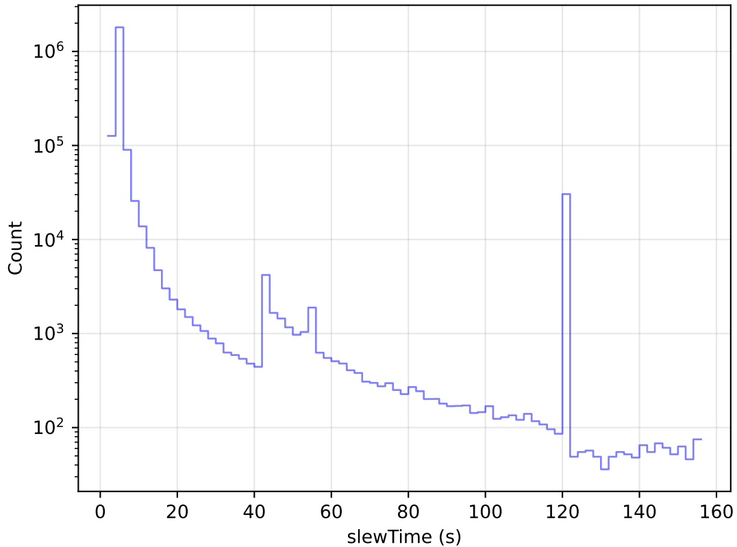
ddf_acor_sf20_lsf30_lsr20_v3.4_10yrs All visits: Slew Time Histogram
