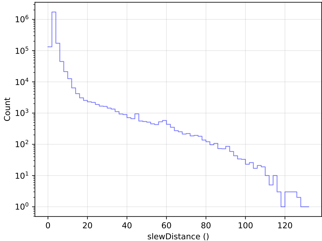
ddf_acor_sf20_lsf30_lsr20_v3.4_10yrs All visits: Slew Distance Histogram
