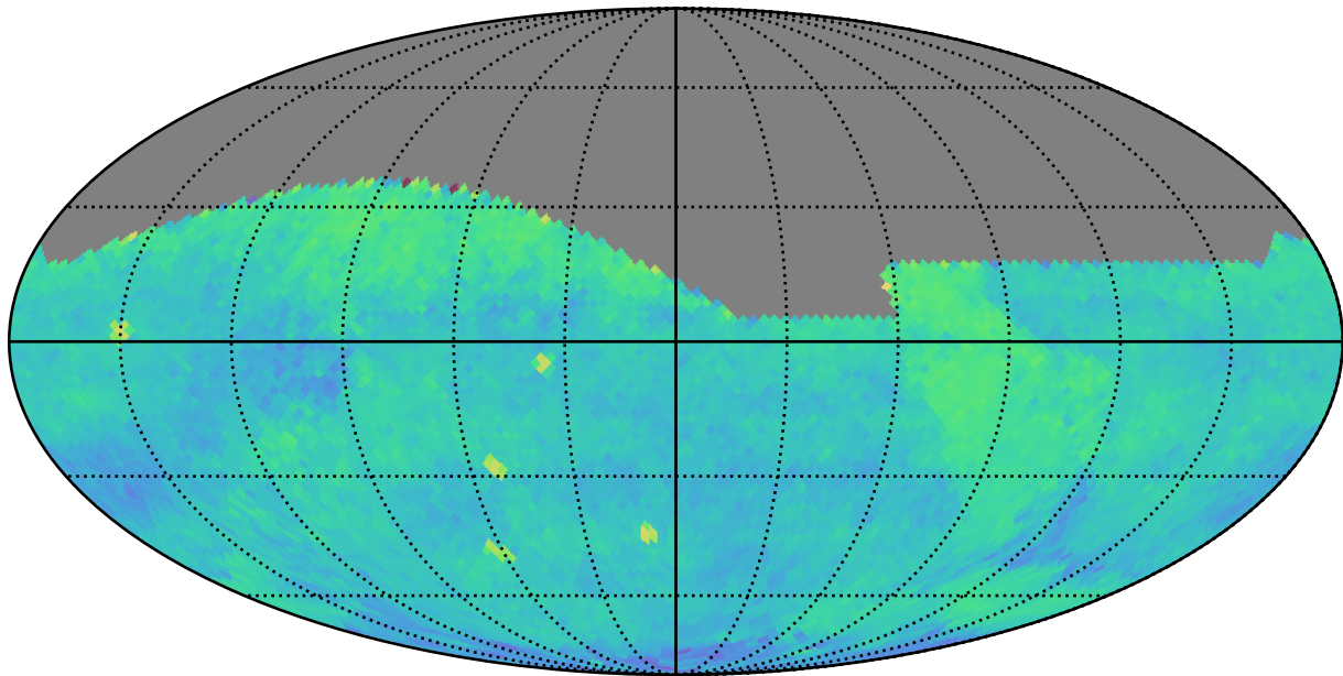
ddf_acor_sf20_lsf30_lsr20_v3.4_10yrs (g or r or i): PairFraction
