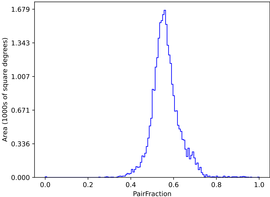
ddf_acor_sf20_lsf30_lsr20_v3.4_10yrs (g or r or i): PairFraction
