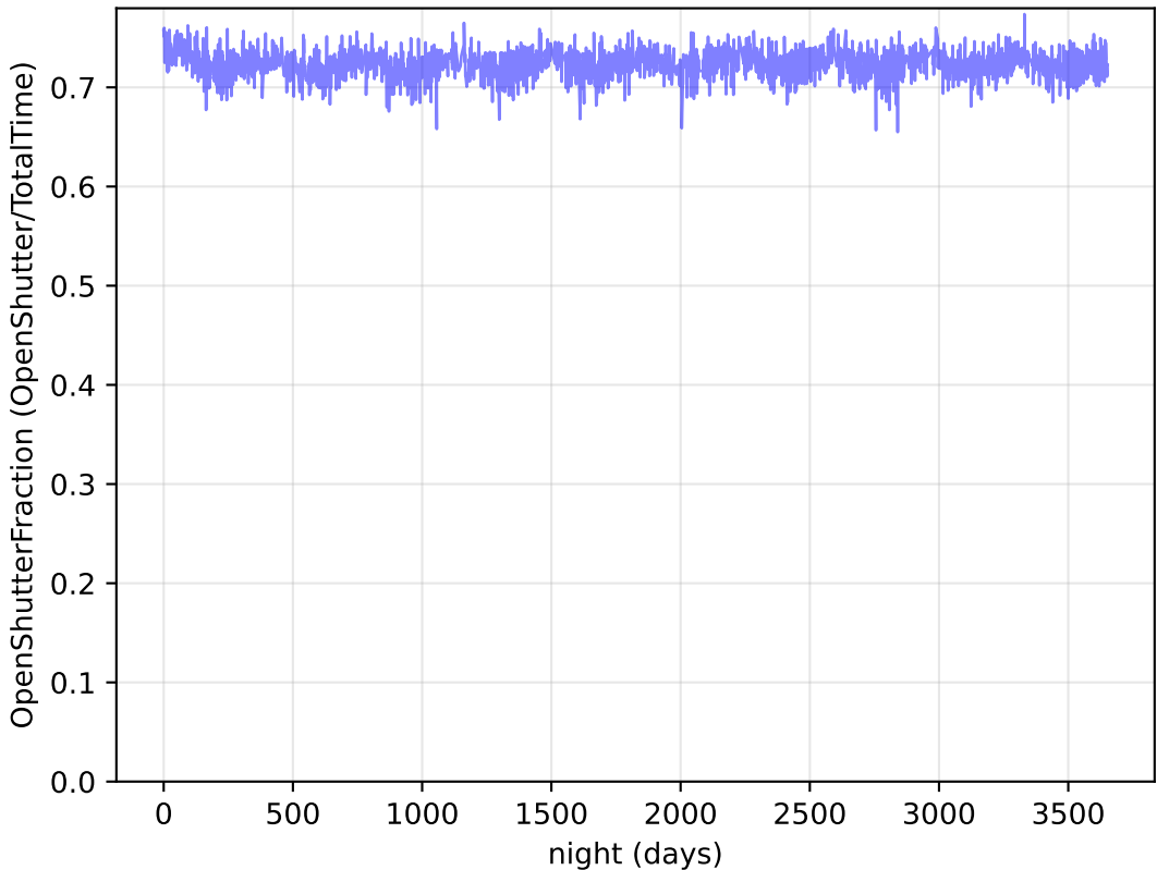
ddf_acor_sf20_lsf30_lsr20_v3.4_10yrs : OpenShutterFraction
