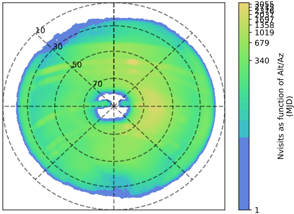
ddf_acor_sf20_lsf30_lsr20_v3.4_10yrs z: Nvisits as function of Alt/Az
