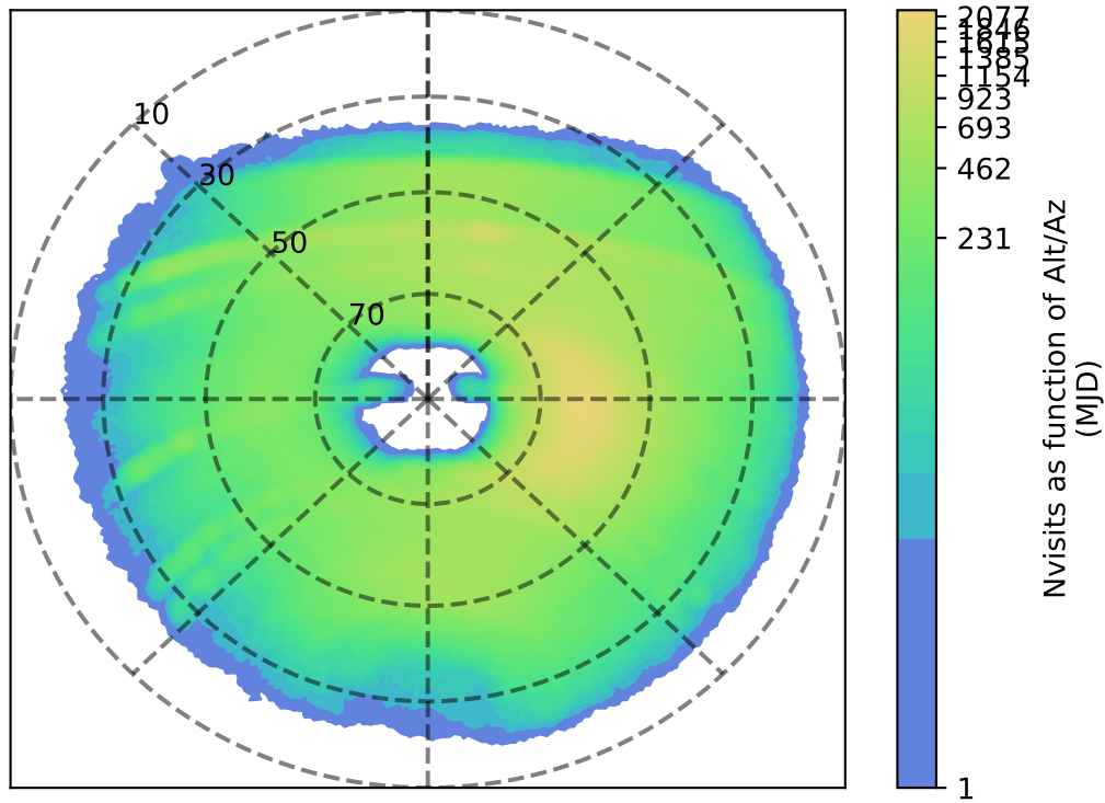
ddf_acor_sf20_lsf30_lsr20_v3.4_10yrs y: Nvisits as function of Alt/Az
