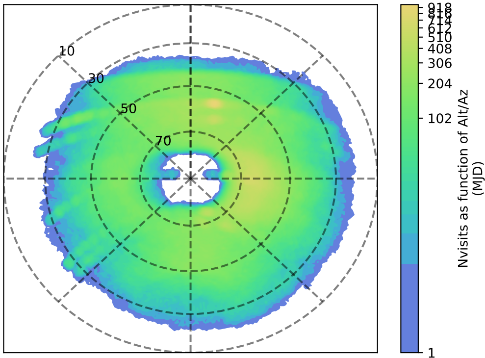
ddf_acor_sf20_lsf30_lsr20_v3.4_10yrs u: Nvisits as function of Alt/Az
