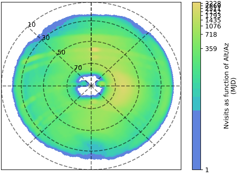
ddf_acor_sf20_lsf30_lsr20_v3.4_10yrs i: Nvisits as function of Alt/Az
