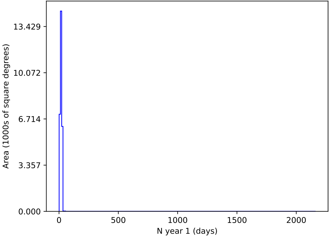
ddf_acor_sf20_lsf30_lsr20_v3.4_10yrs i and night < 365: N year 1
