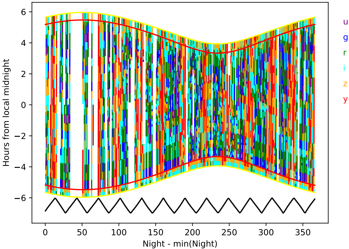
ddf_acor_sf20_lsf30_lsr20_v3.4_10yrs year 8-9: Hourglass
